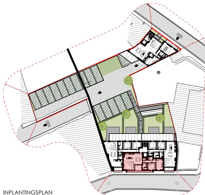
INPLANTINGSPLAN
