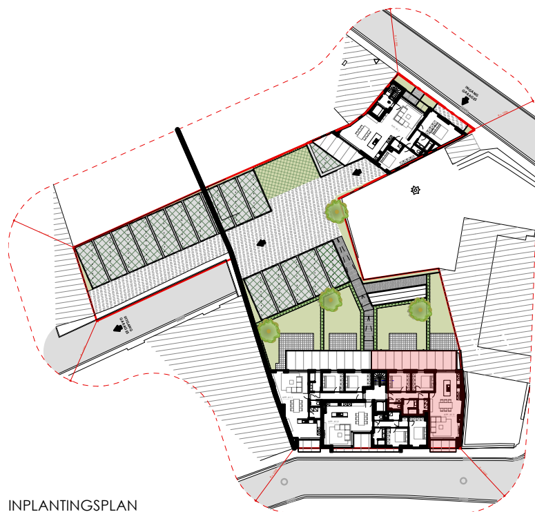
INPLANTINGSPLAN
